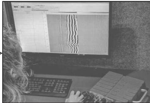
Winlogger Software
